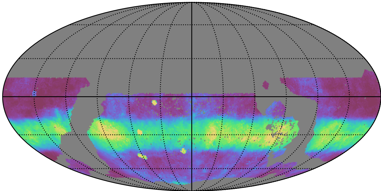
too_elab_r8_d2_gz_v3.4_10yrs WFD r band: Median normairmass
