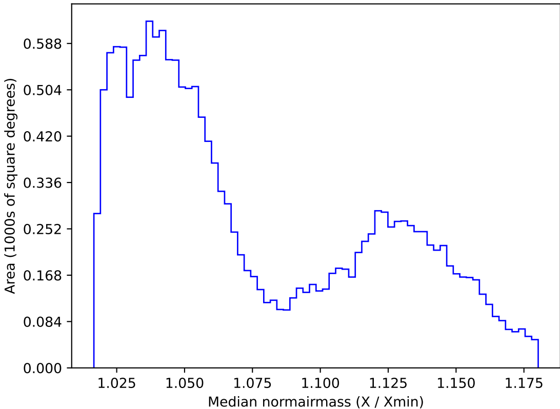
too_elab_r8_d2_gz_v3.4_10yrs WFD r band: Median normairmass
