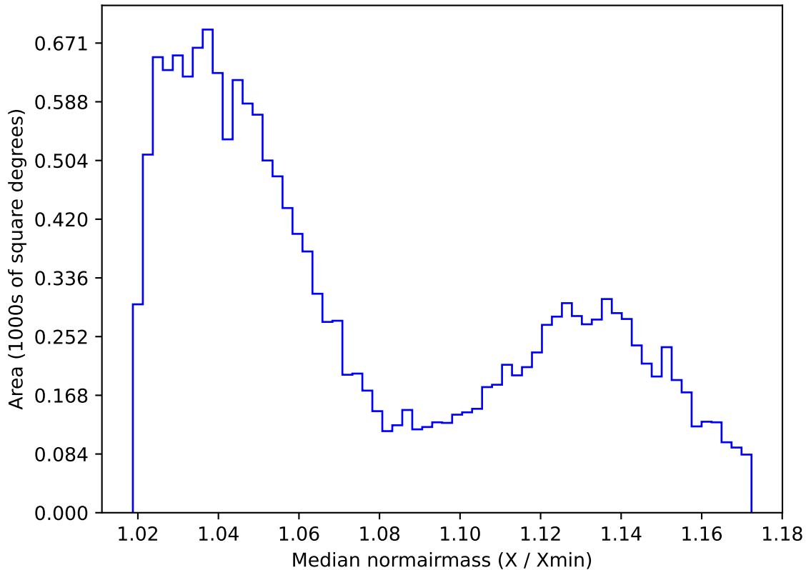
too_elab_r8_d2_gz_v3.4_10yrs WFD i band: Median normairmass
