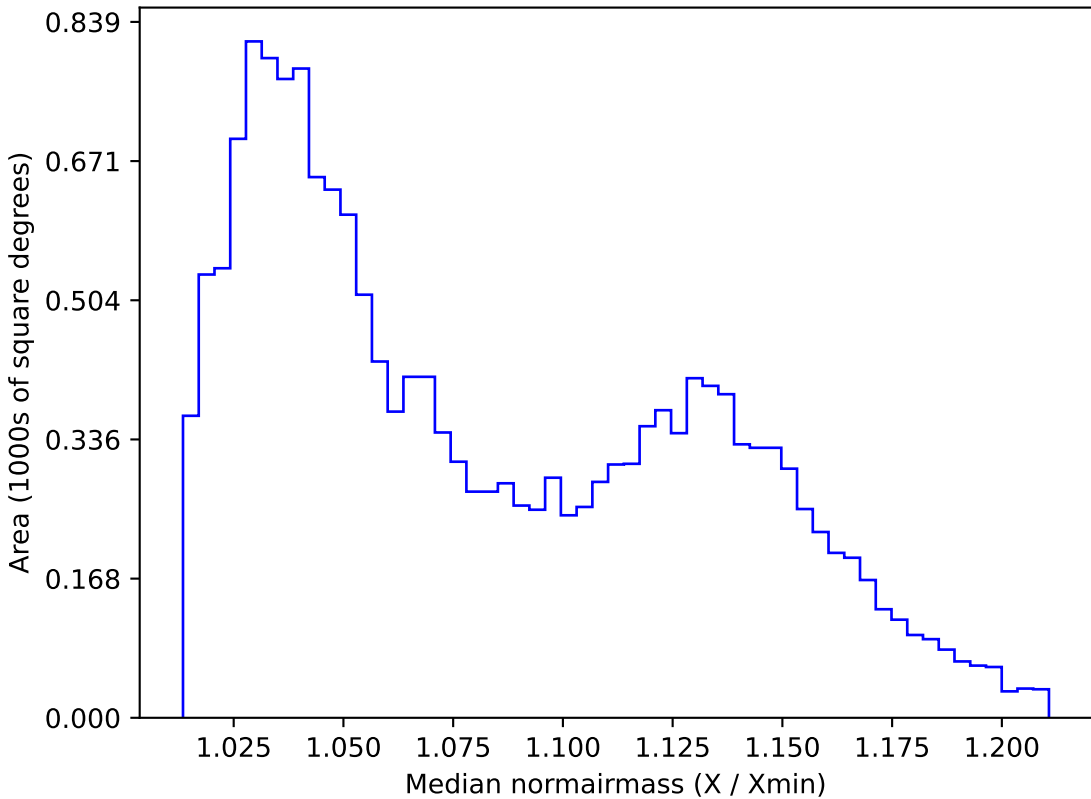
too_elab_r8_d2_gz_v3.4_10yrs WFD g band: Median normairmass
