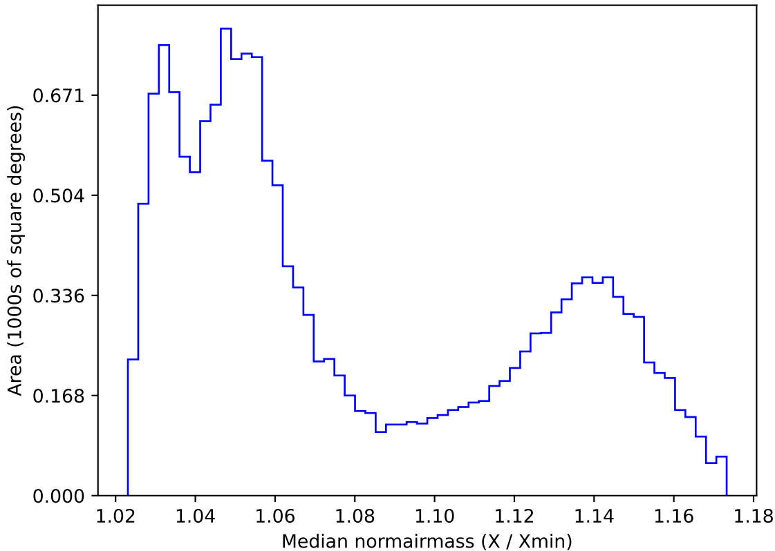
too_elab_r8_d2_gz_v3.4_10yrs WFD all bands: Median normairmass
