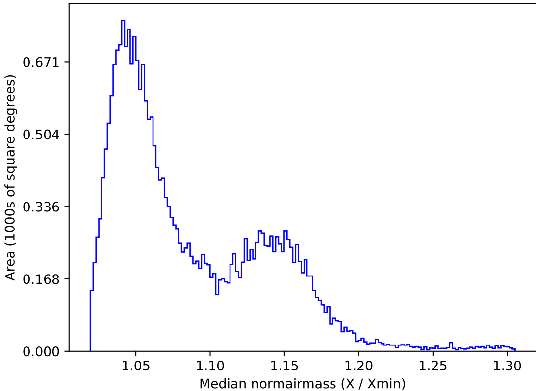
too_elab_r8_d2_gz_v3.4_10yrs All sky z band: Median normairmass
