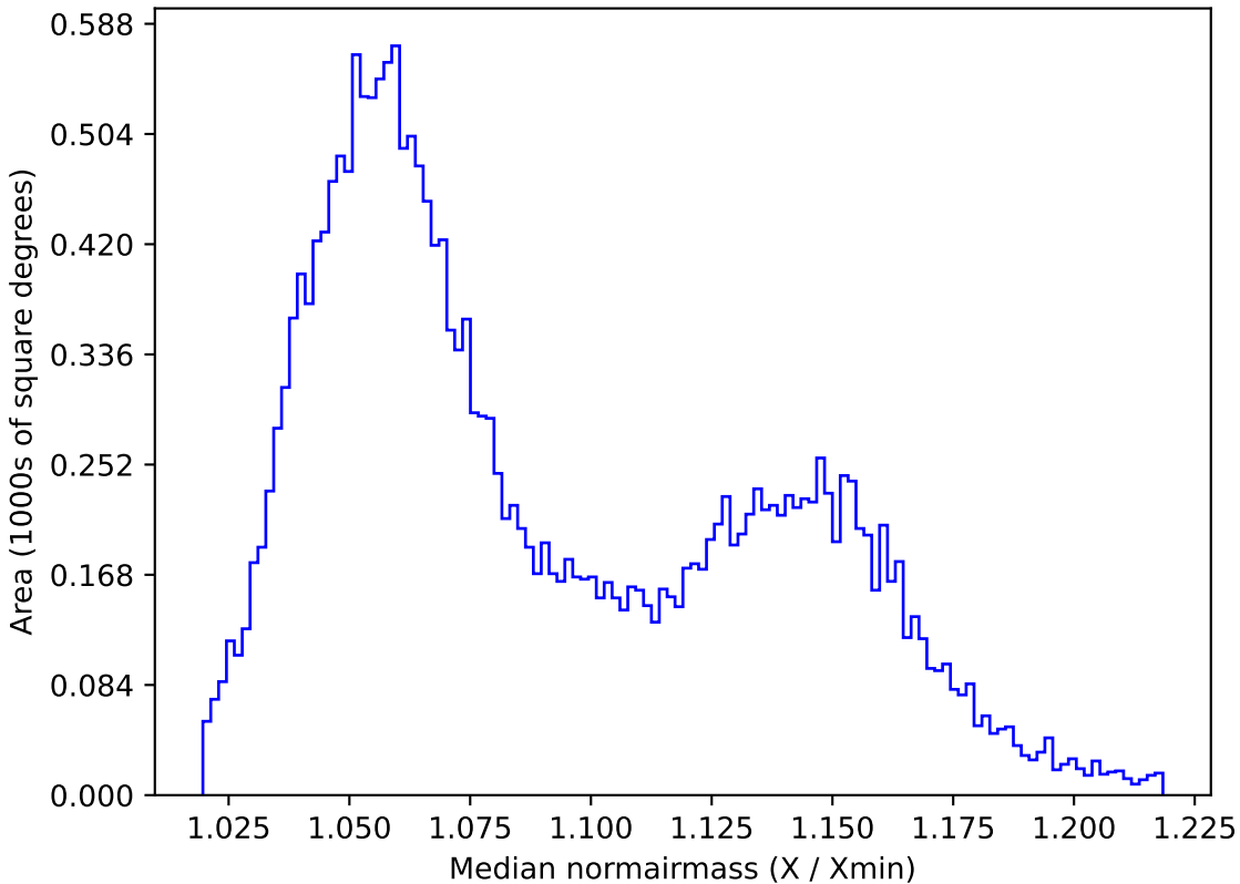
too_elab_r8_d2_gz_v3.4_10yrs All sky y band: Median normairmass
