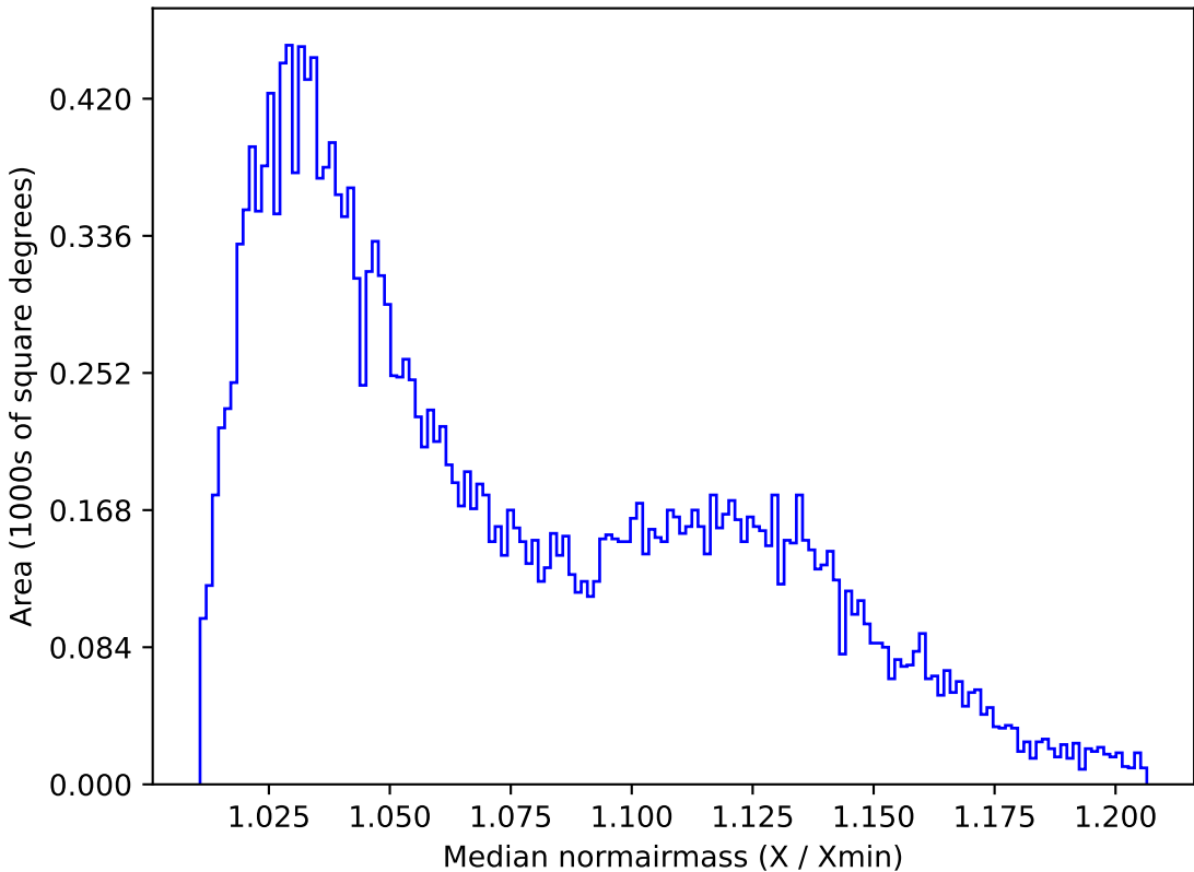
too_elab_r8_d2_gz_v3.4_10yrs All sky u band: Median normairmass
