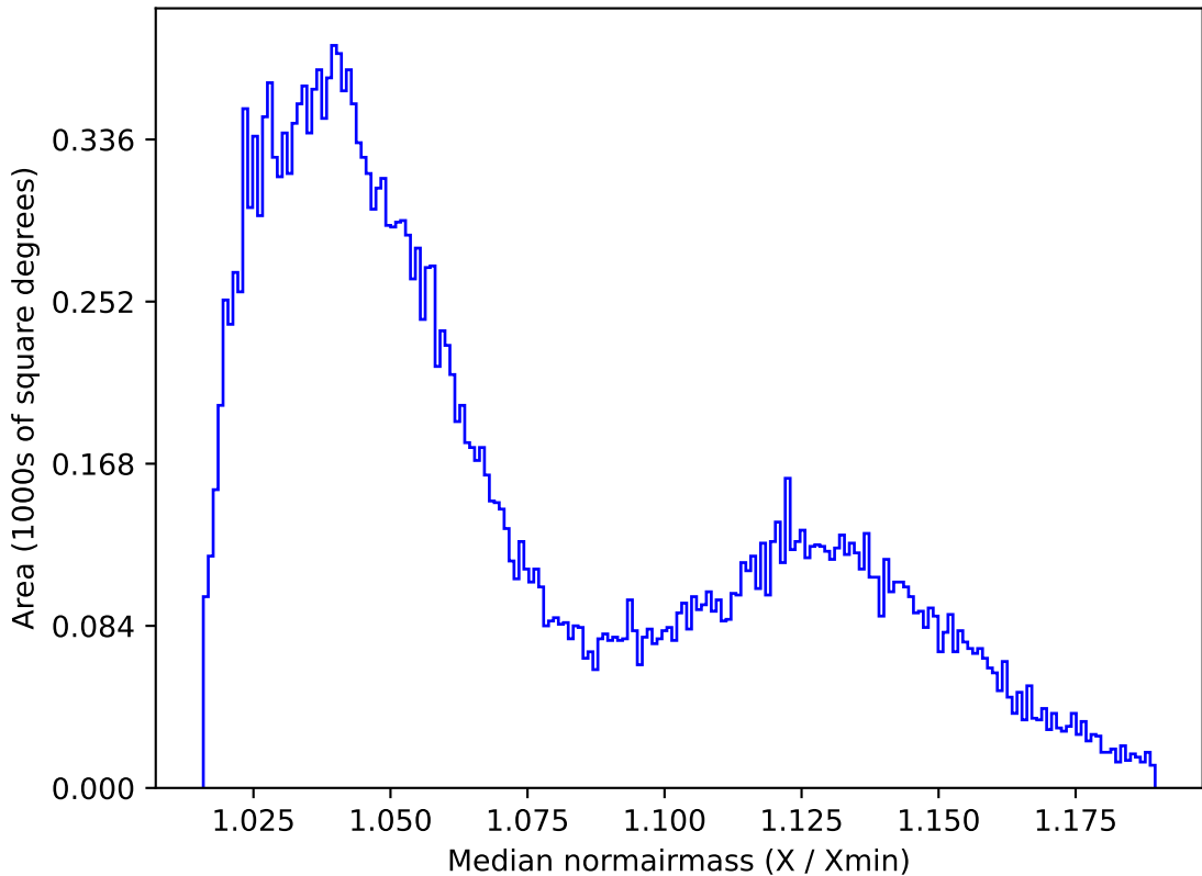
too_elab_r8_d2_gz_v3.4_10yrs All sky r band: Median normairmass
