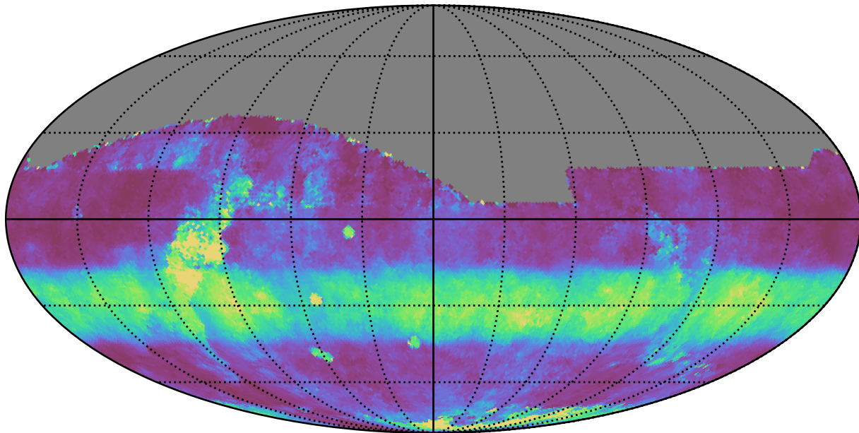
too_elab_r8_d2_gz_v3.4_10yrs All sky i band: Median normairmass
