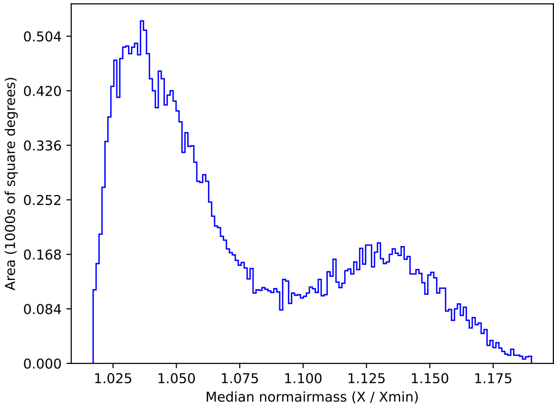
too_elab_r8_d2_gz_v3.4_10yrs All sky i band: Median normairmass
