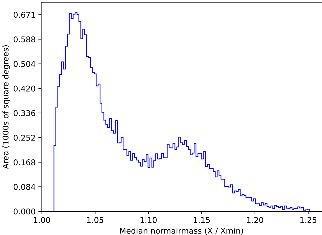
too_elab_r8_d2_gz_v3.4_10yrs All sky g band: Median normairmass
