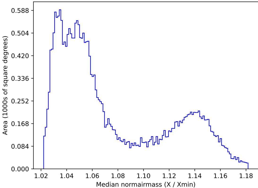
too_elab_r8_d2_gz_v3.4_10yrs All sky all bands: Median normairmass
