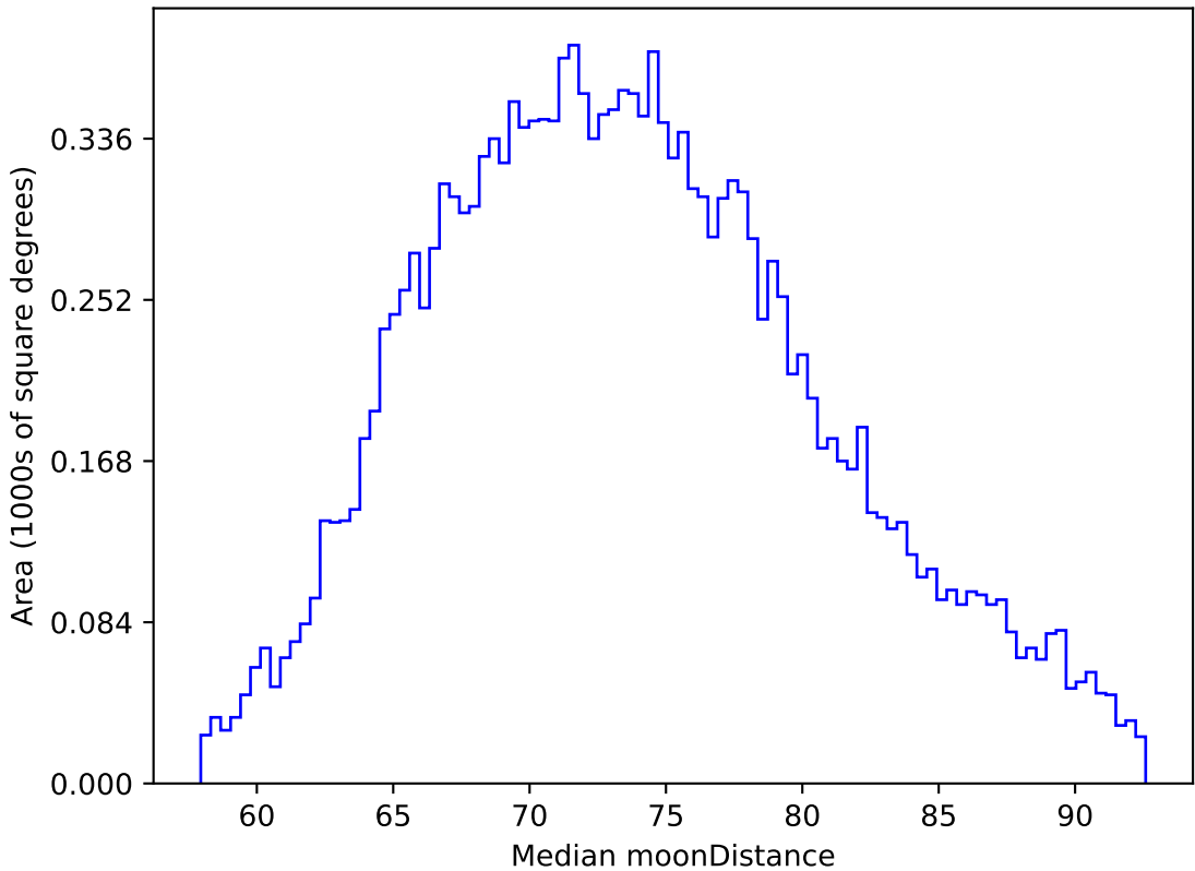
too_elab_r8_d2_gz_v3.4_10yrs WFD z band: Median moonDistance
