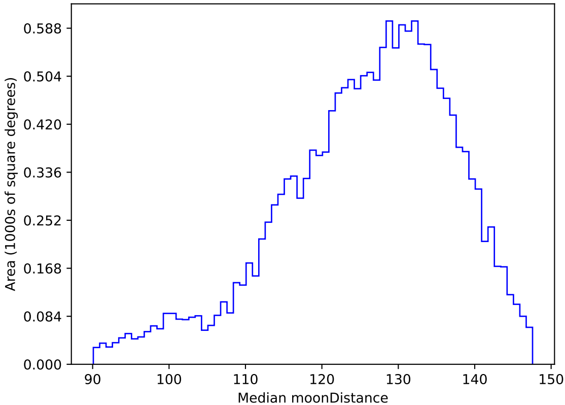
too_elab_r8_d2_gz_v3.4_10yrs WFD u band: Median moonDistance
