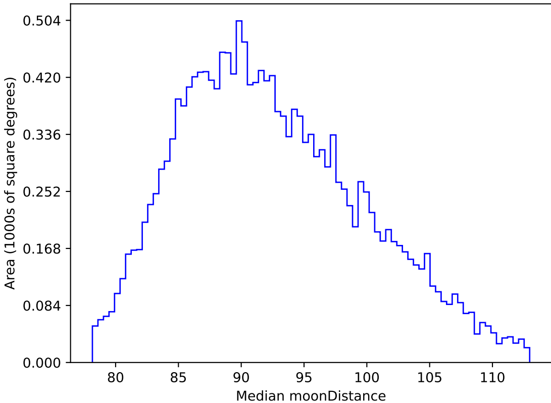
too_elab_r8_d2_gz_v3.4_10yrs WFD i band: Median moonDistance
