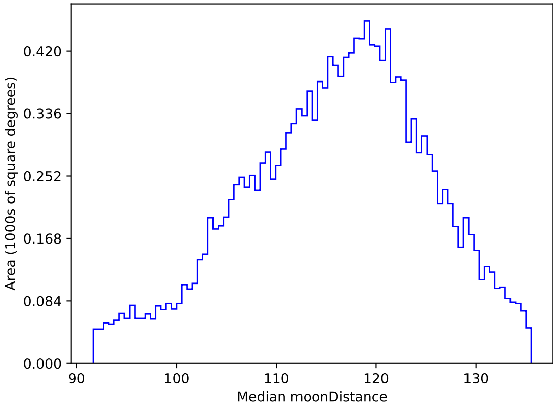
too_elab_r8_d2_gz_v3.4_10yrs WFD g band: Median moonDistance
