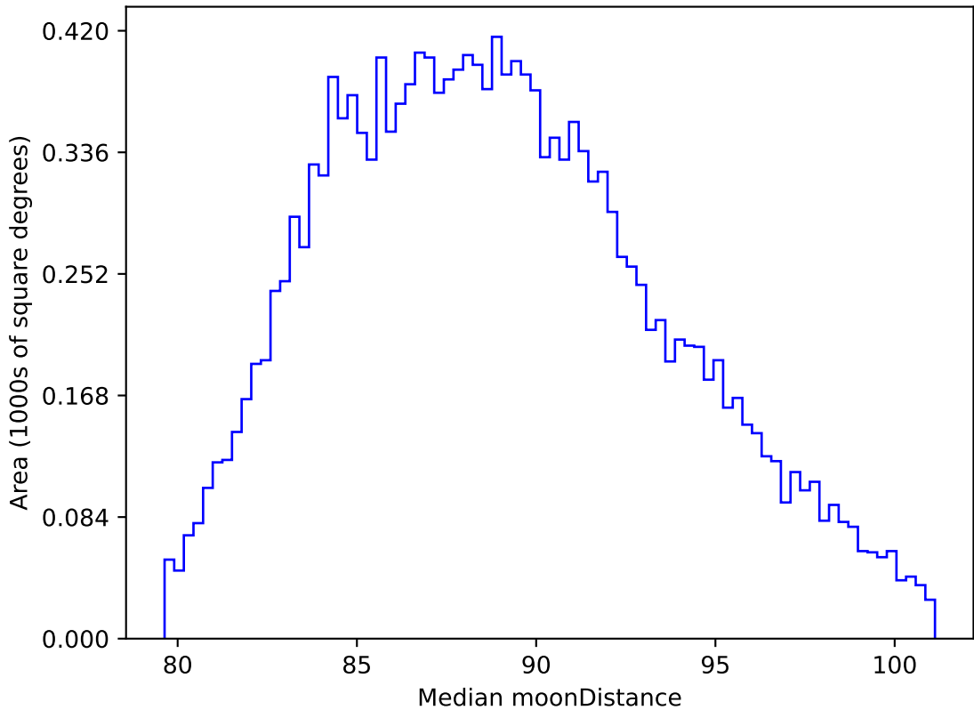
too_elab_r8_d2_gz_v3.4_10yrs WFD all bands: Median moonDistance
