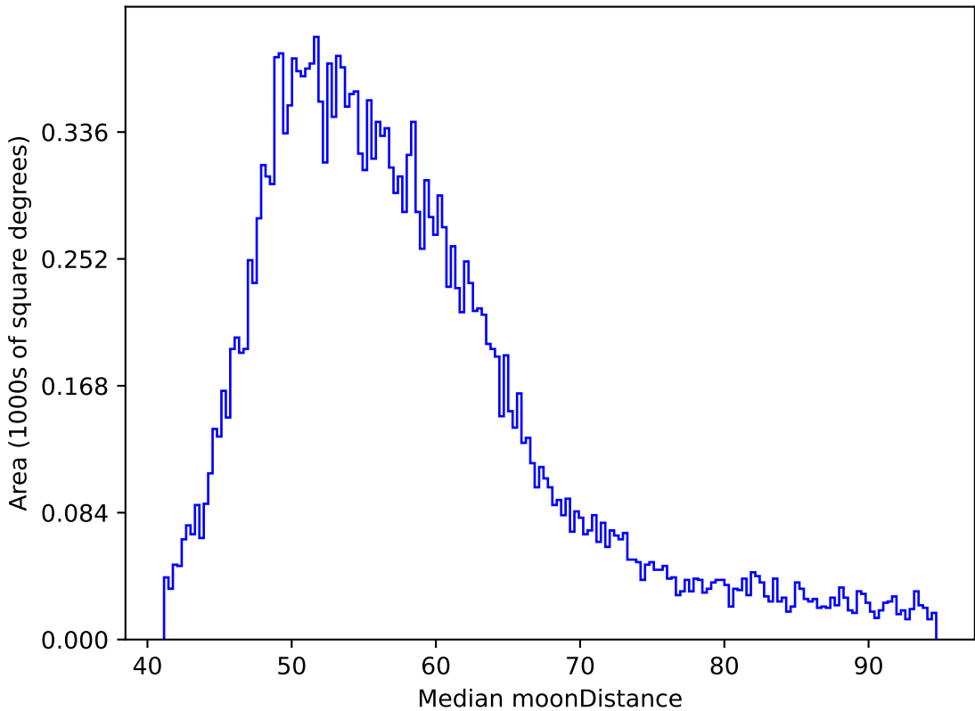
too_elab_r8_d2_gz_v3.4_10yrs All sky y band: Median moonDistance
