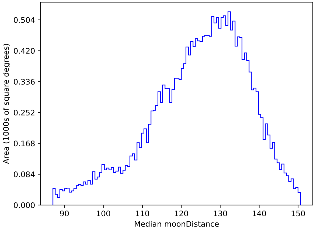
too_elab_r8_d2_gz_v3.4_10yrs All sky u band: Median moonDistance
