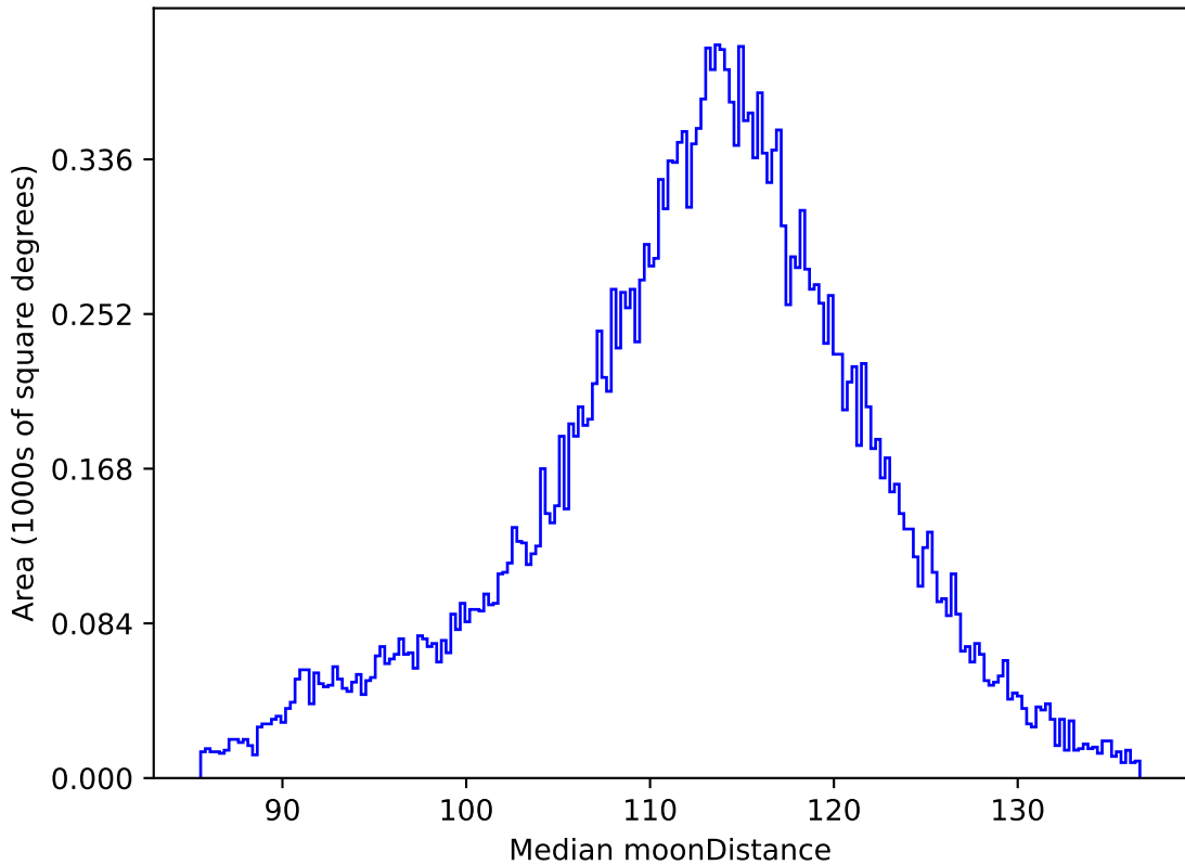
too_elab_r8_d2_gz_v3.4_10yrs All sky r band: Median moonDistance
