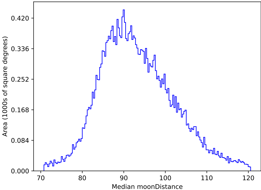
too_elab_r8_d2_gz_v3.4_10yrs All sky i band: Median moonDistance
