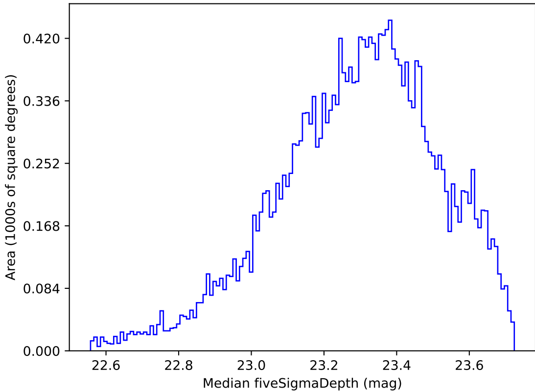
too_elab_r8_d2_gz_v3.4_10yrs Yr 1 u band: Median fiveSigmaDepth
