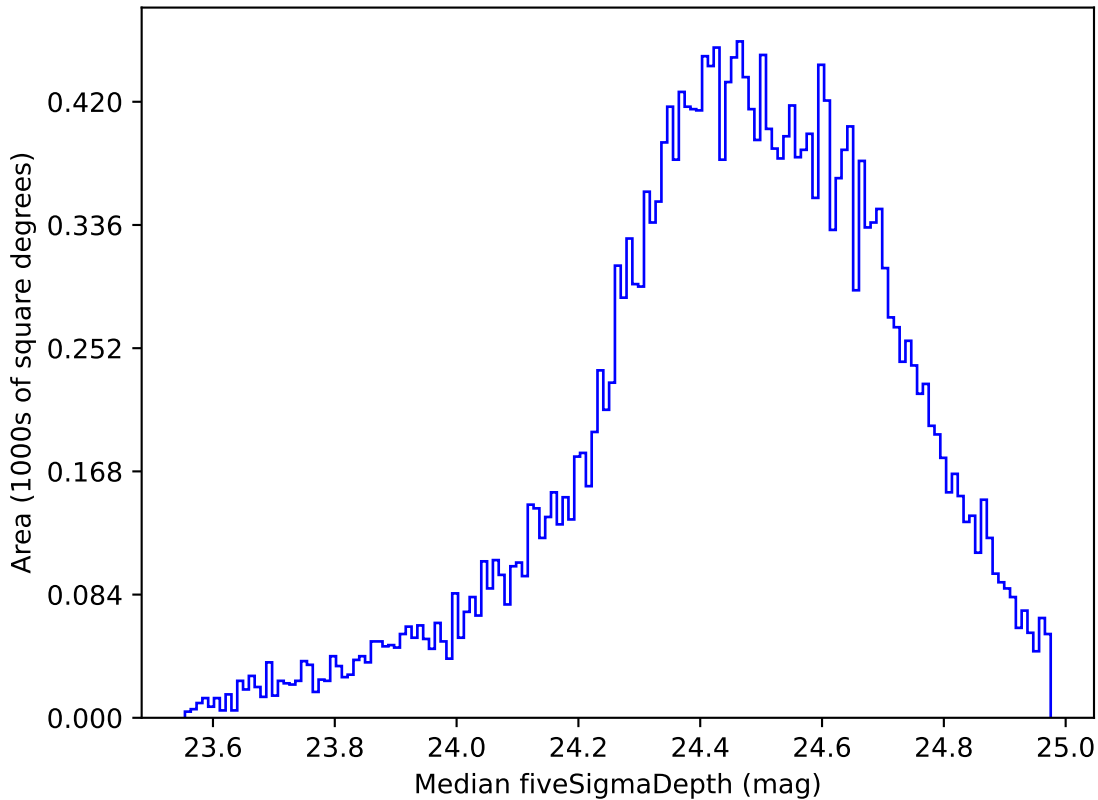
too_elab_r8_d2_gz_v3.4_10yrs Yr 1 g band: Median fiveSigmaDepth
