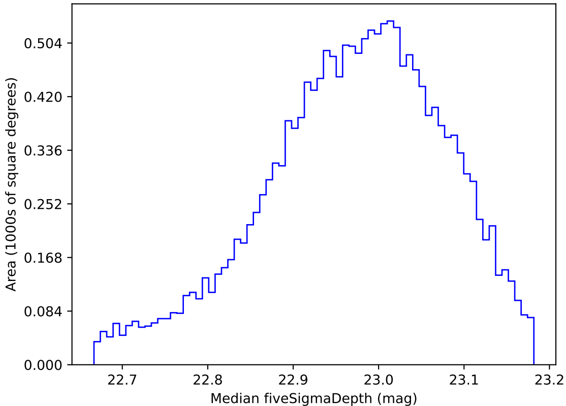
too_elab_r8_d2_gz_v3.4_10yrs WFD z band: Median fiveSigmaDepth
