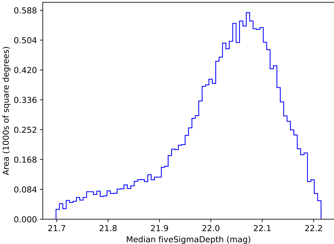
too_elab_r8_d2_gz_v3.4_10yrs WFD y band: Median fiveSigmaDepth
