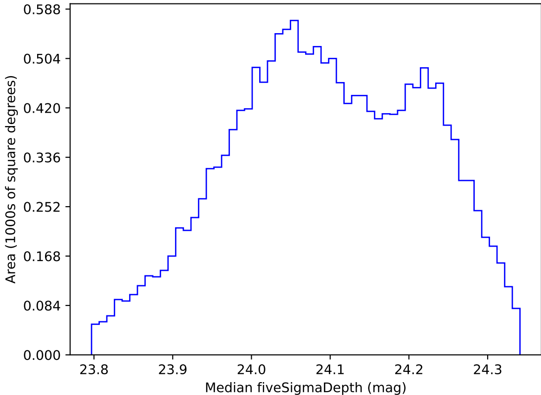
too_elab_r8_d2_gz_v3.4_10yrs WFD r band: Median fiveSigmaDepth
