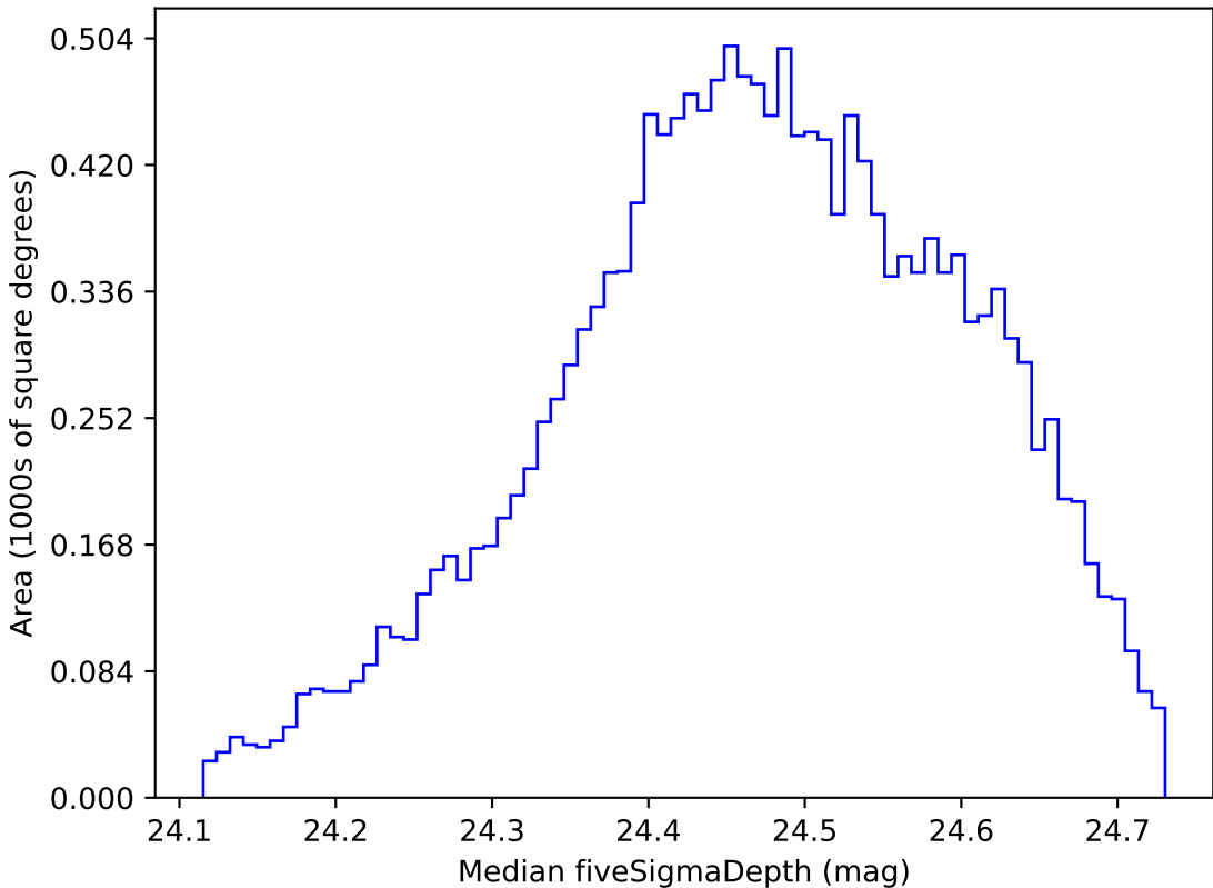
too_elab_r8_d2_gz_v3.4_10yrs WFD g band: Median fiveSigmaDepth
