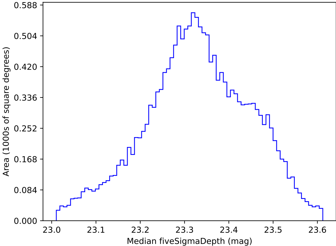
too_elab_r8_d2_gz_v3.4_10yrs WFD all bands: Median fiveSigmaDepth
