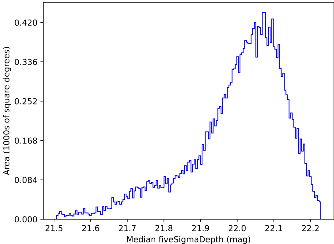
too_elab_r8_d2_gz_v3.4_10yrs All sky y band: Median fiveSigmaDepth
