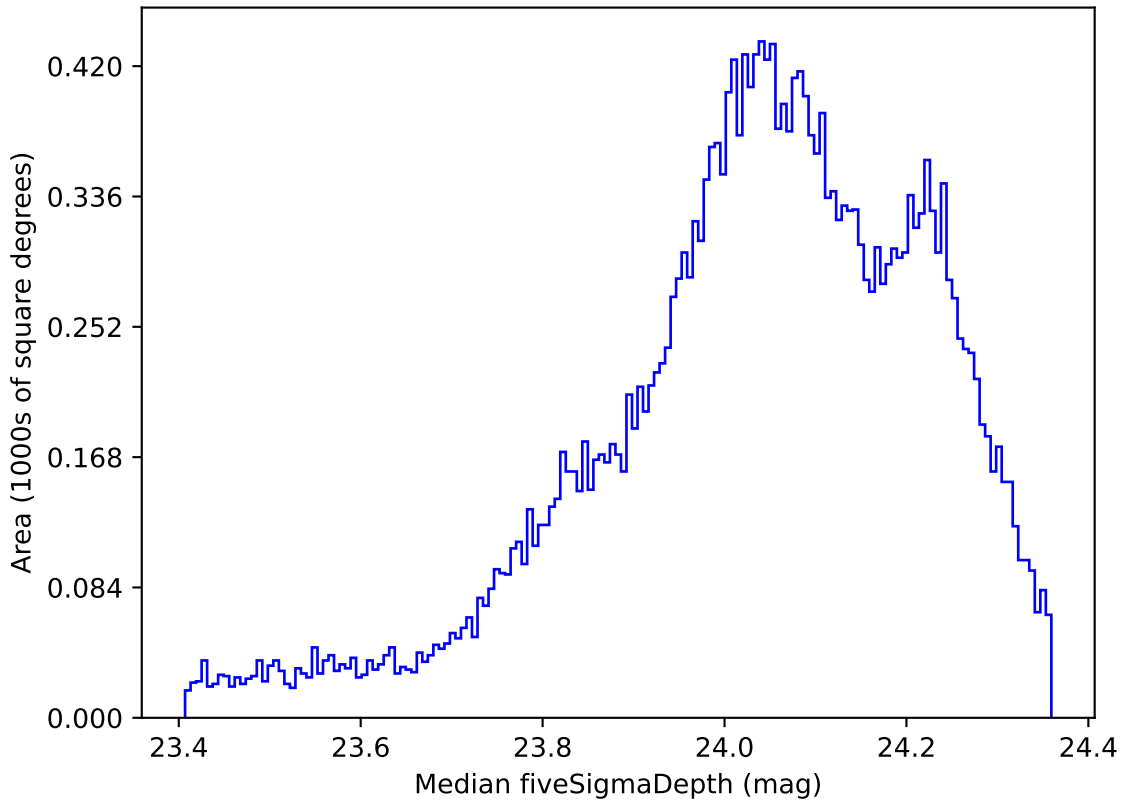
too_elab_r8_d2_gz_v3.4_10yrs All sky r band: Median fiveSigmaDepth
