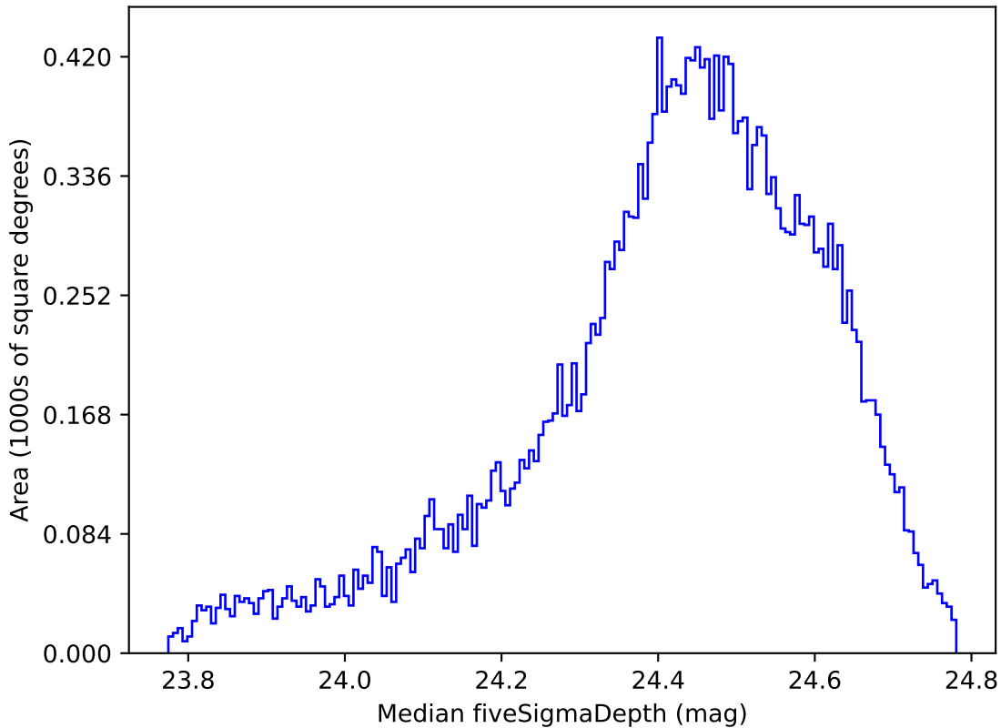
too_elab_r8_d2_gz_v3.4_10yrs All sky g band: Median fiveSigmaDepth
