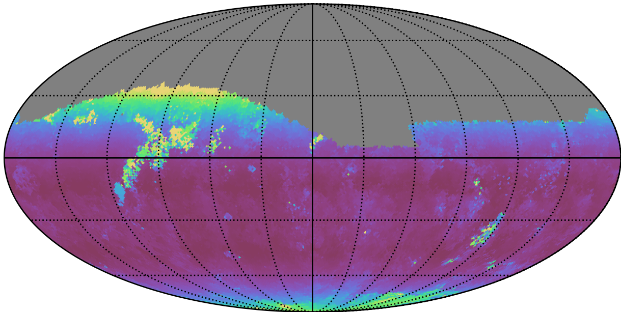
too_elab_r8_d2_gz_v3.4_10yrs Yr 1 z band: Median airmass
