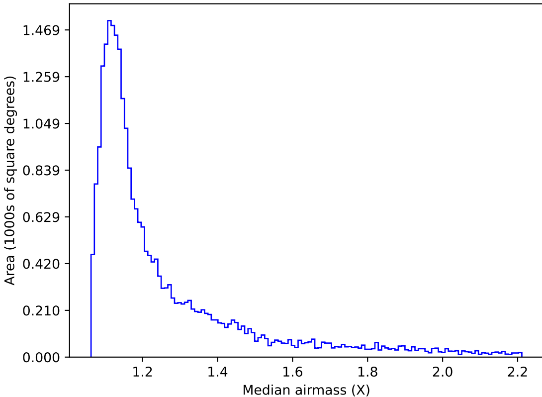
too_elab_r8_d2_gz_v3.4_10yrs Yr 1 z band: Median airmass
