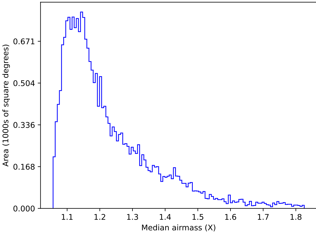
too_elab_r8_d2_gz_v3.4_10yrs Yr 1 u band: Median airmass
