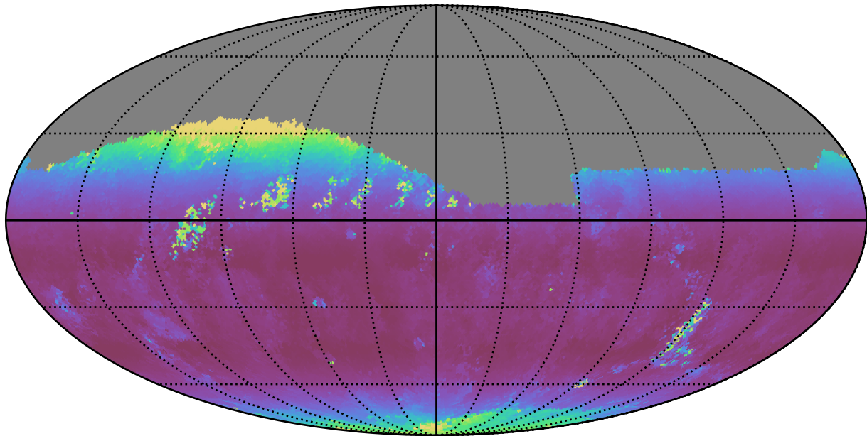
too_elab_r8_d2_gz_v3.4_10yrs Yr 1 r band: Median airmass
