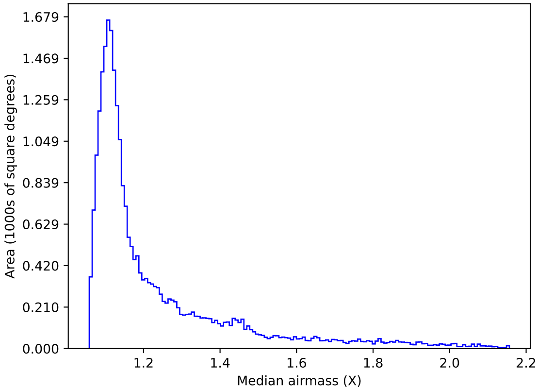
too_elab_r8_d2_gz_v3.4_10yrs Yr 1 i band: Median airmass
