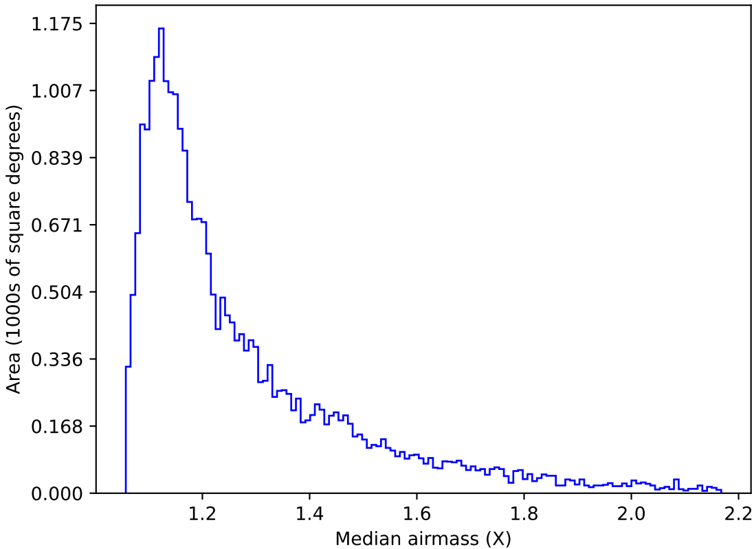
too_elab_r8_d2_gz_v3.4_10yrs Yr 1 g band: Median airmass
