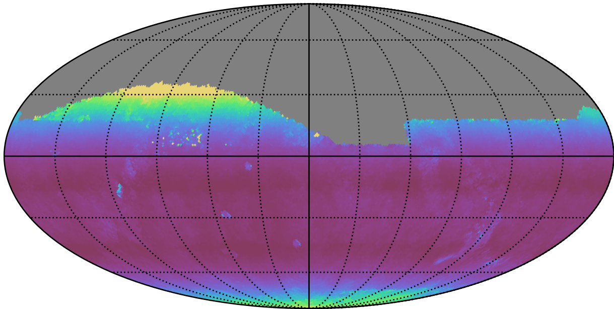
too_elab_r8_d2_gz_v3.4_10yrs Yr 1 all bands: Median airmass
