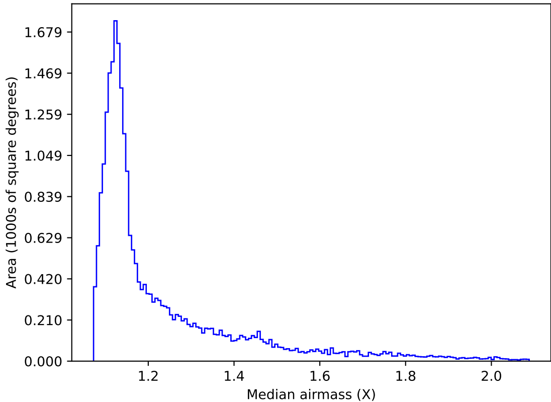
too_elab_r8_d2_gz_v3.4_10yrs Yr 1 all bands: Median airmass
