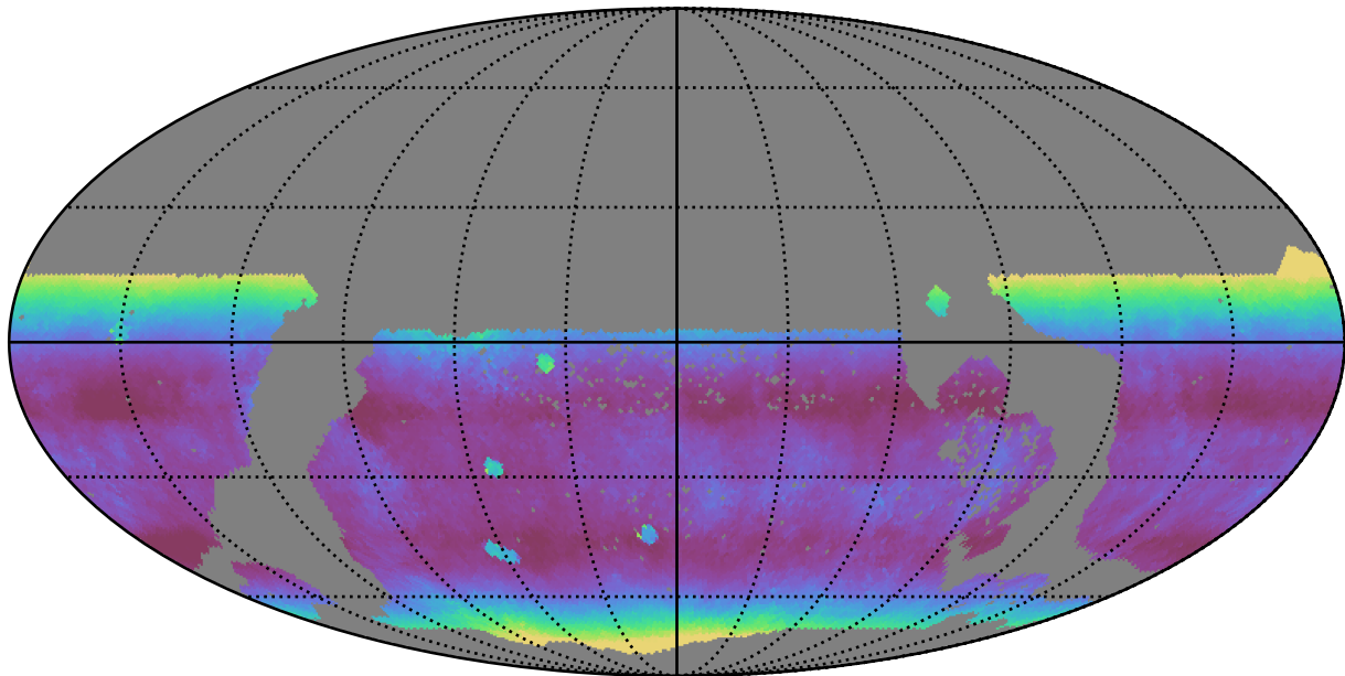
too_elab_r8_d2_gz_v3.4_10yrs WFD z band: Median airmass
