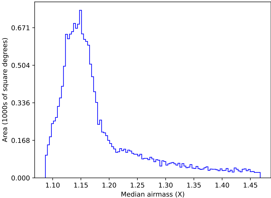
too_elab_r8_d2_gz_v3.4_10yrs WFD z band: Median airmass
