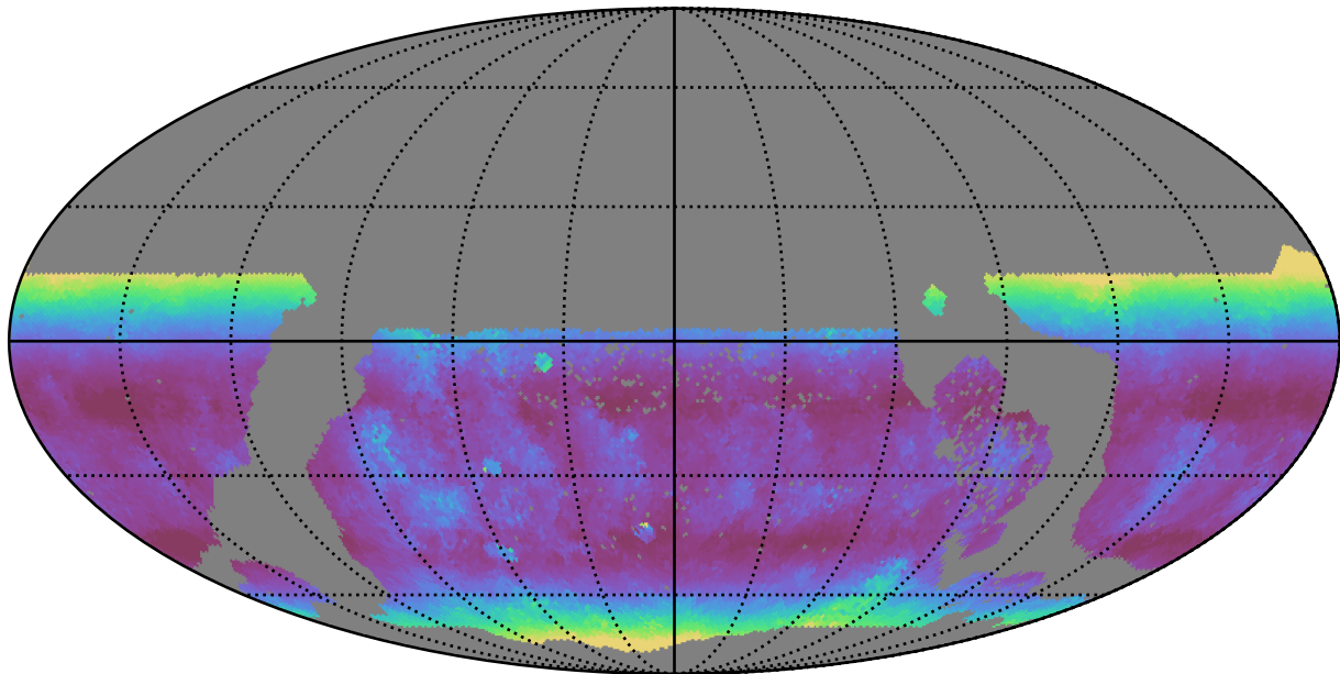
too_elab_r8_d2_gz_v3.4_10yrs WFD u band: Median airmass
