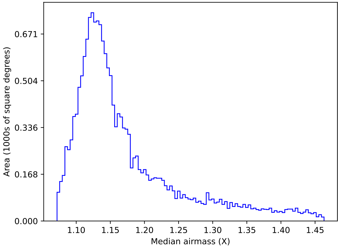
too_elab_r8_d2_gz_v3.4_10yrs WFD u band: Median airmass
