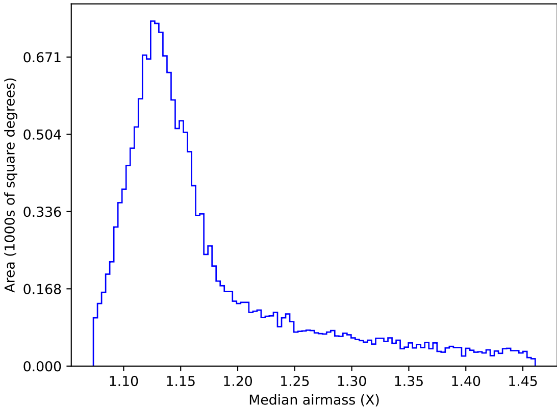
too_elab_r8_d2_gz_v3.4_10yrs WFD r band: Median airmass
