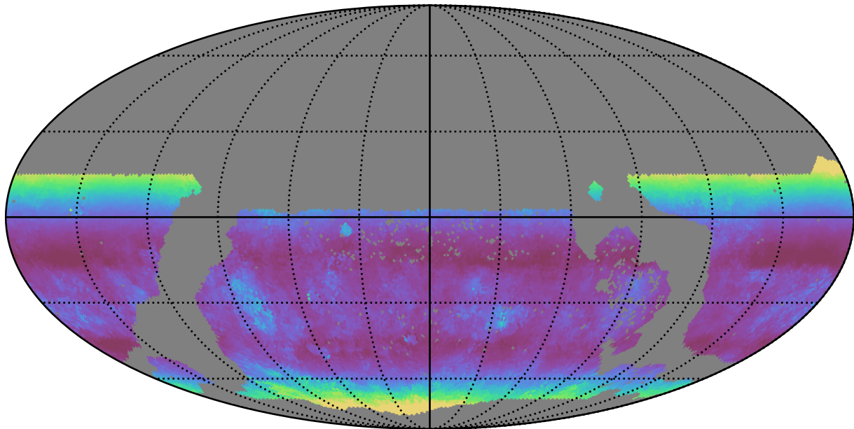
too_elab_r8_d2_gz_v3.4_10yrs WFD g band: Median airmass
