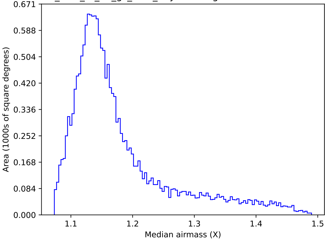
too_elab_r8_d2_gz_v3.4_10yrs WFD g band: Median airmass
