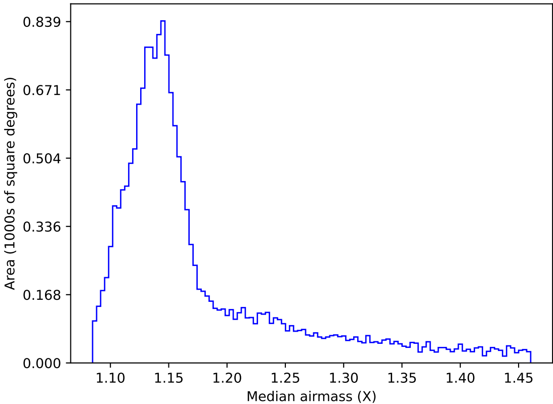
too_elab_r8_d2_gz_v3.4_10yrs WFD all bands: Median airmass
