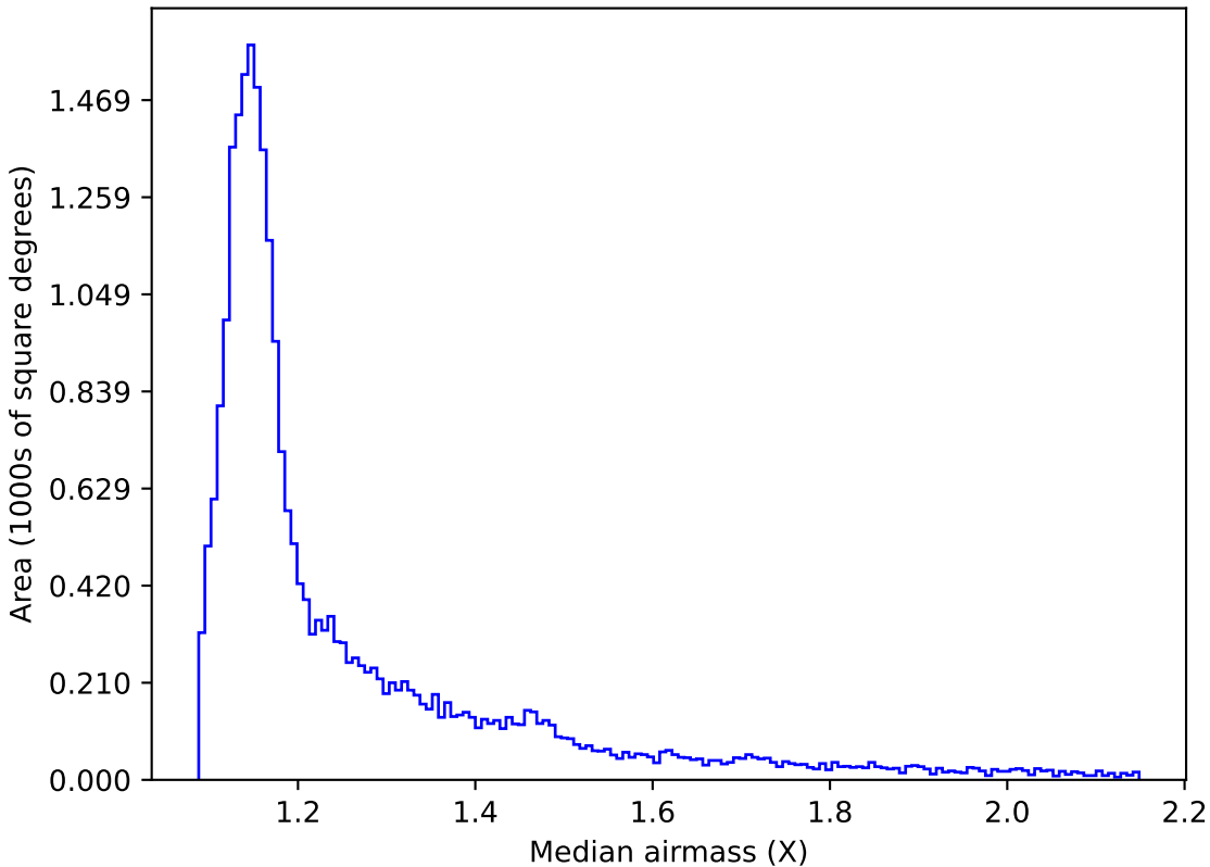
too_elab_r8_d2_gz_v3.4_10yrs All sky z band: Median airmass
