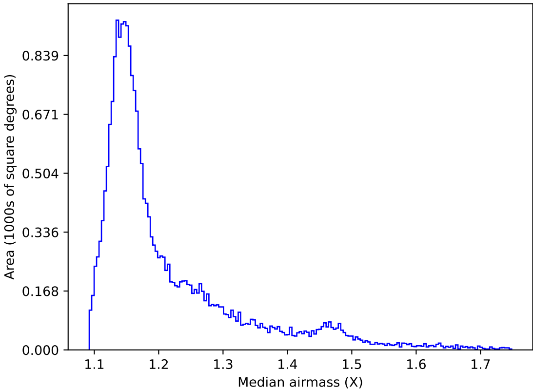
too_elab_r8_d2_gz_v3.4_10yrs All sky y band: Median airmass
